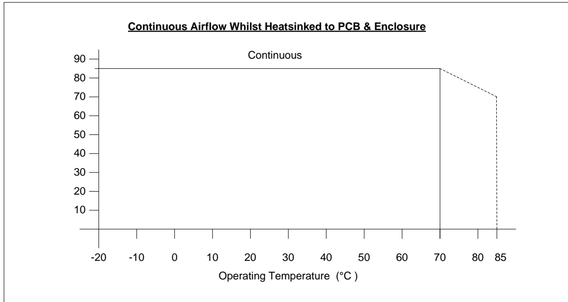
Figure 11: Operating Temperature
